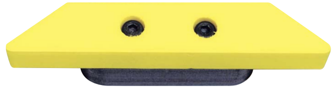
57956 Raised Panel Pad Assembly (pad, adapter for mounting to tool, two mounting screws).
